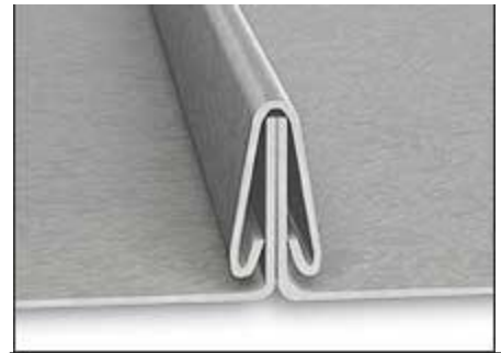
1" BATTEN SEAM AFTER SEAMING
